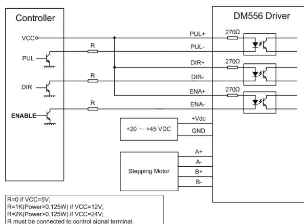
Figure 9: Typical connection
