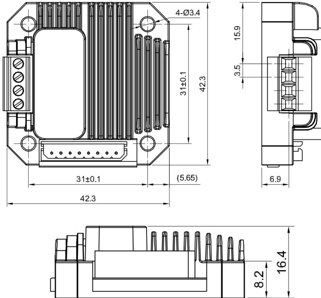
Figure 1: Mechanical specifications
