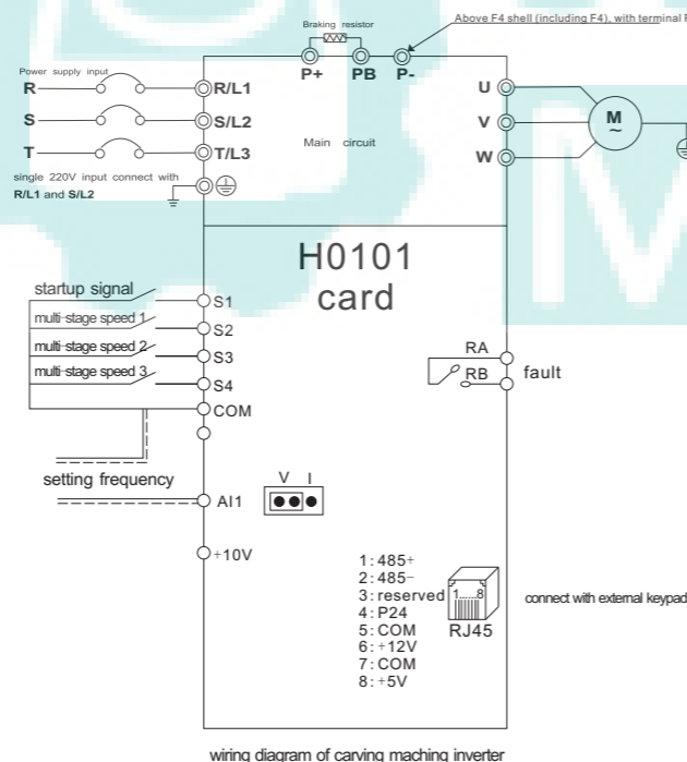
wiring diagram of carving machine inverter
