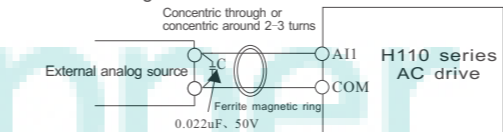
Wiring diagram of analog input terminal plus filter processing
