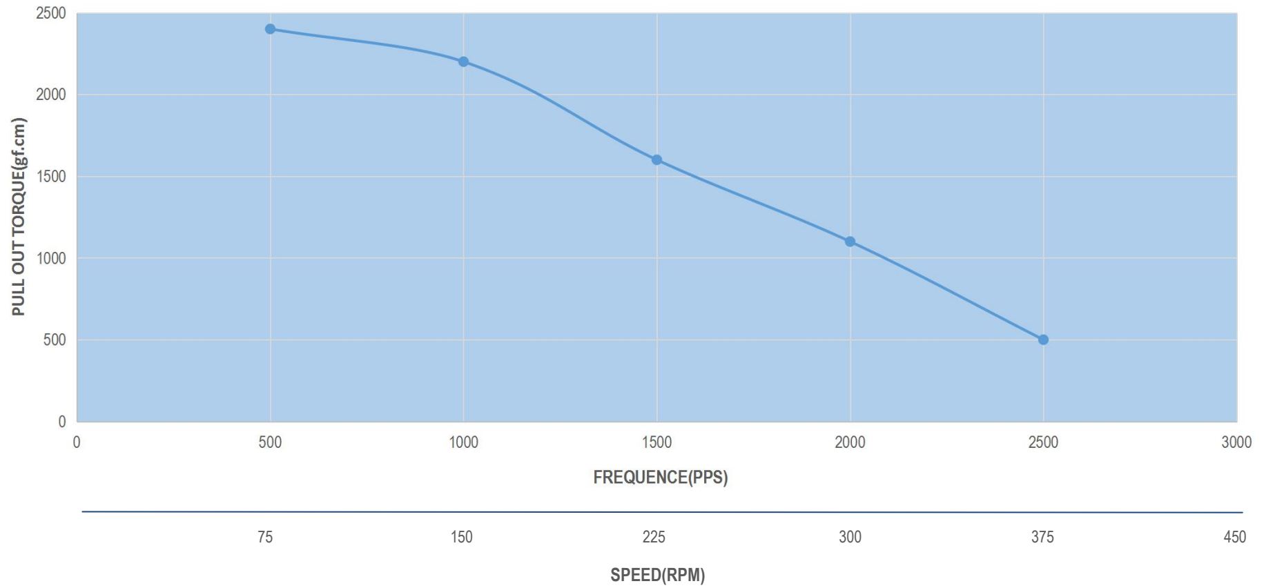
17HS19-0406S PULL OUT TORQUE ( 0.4A/PHASE 24V CONSTANT CURRENT HALF STEP )
