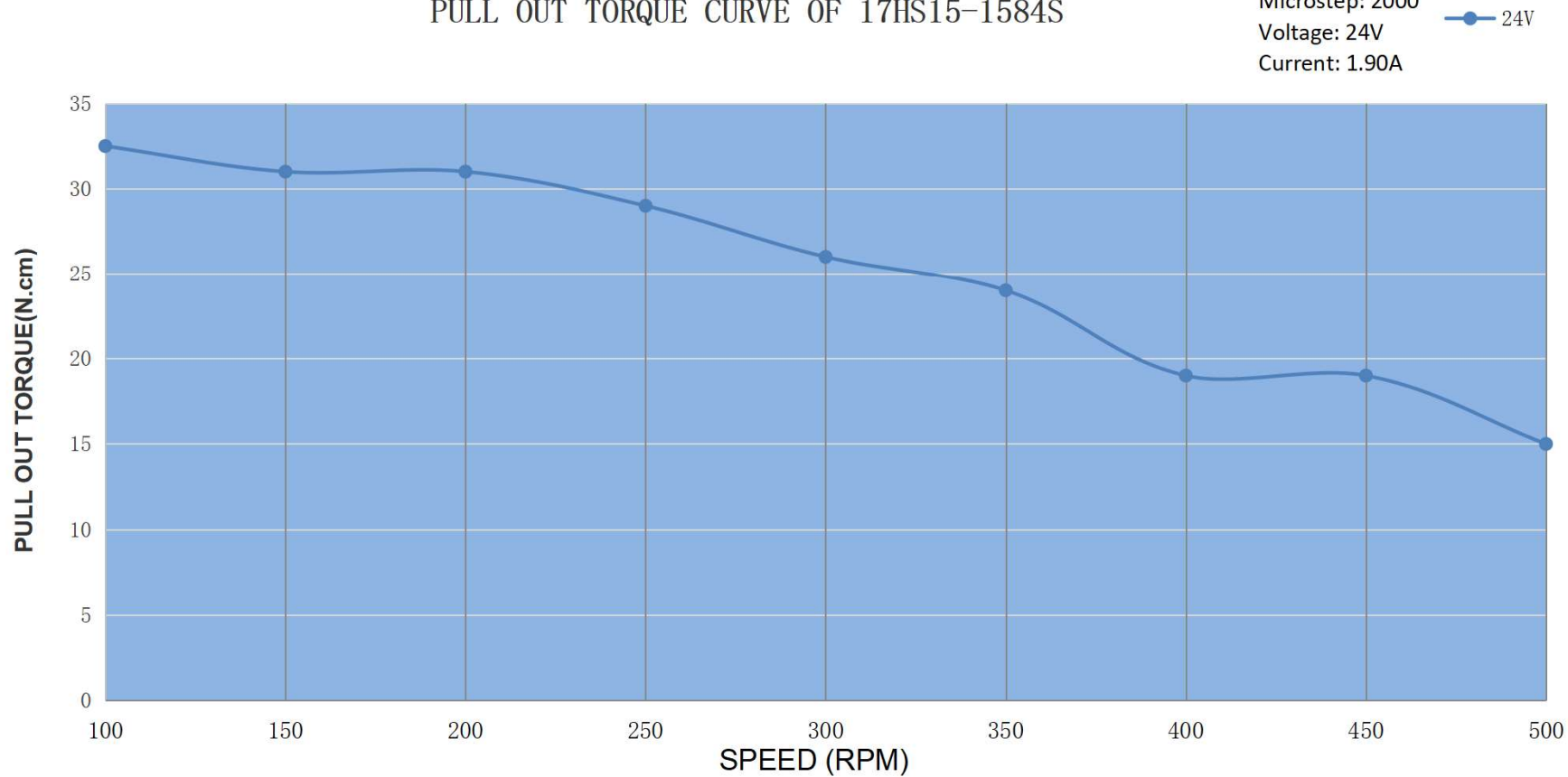
PULL OUT TORQUE CURVE OF 17HS15-1584S
